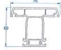
Casement Mullion
