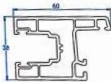
Sliding Sash 60
