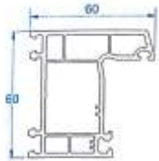
Casement Frame 60
