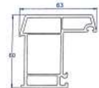
False Mullion
