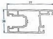
Sliding Sash 80
