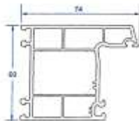
Casement Frame 74
