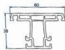
Sliding Sash Mullion
