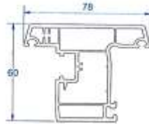
Casement Sash
