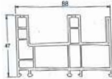
Sliding Frame 2.5 Track (WOT-47)
