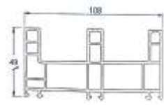
Sliding Frame 3 Track (WOT-49)
