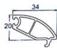
Casement Single Bead
